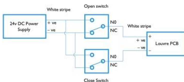
Single Switch Panel Wiring
